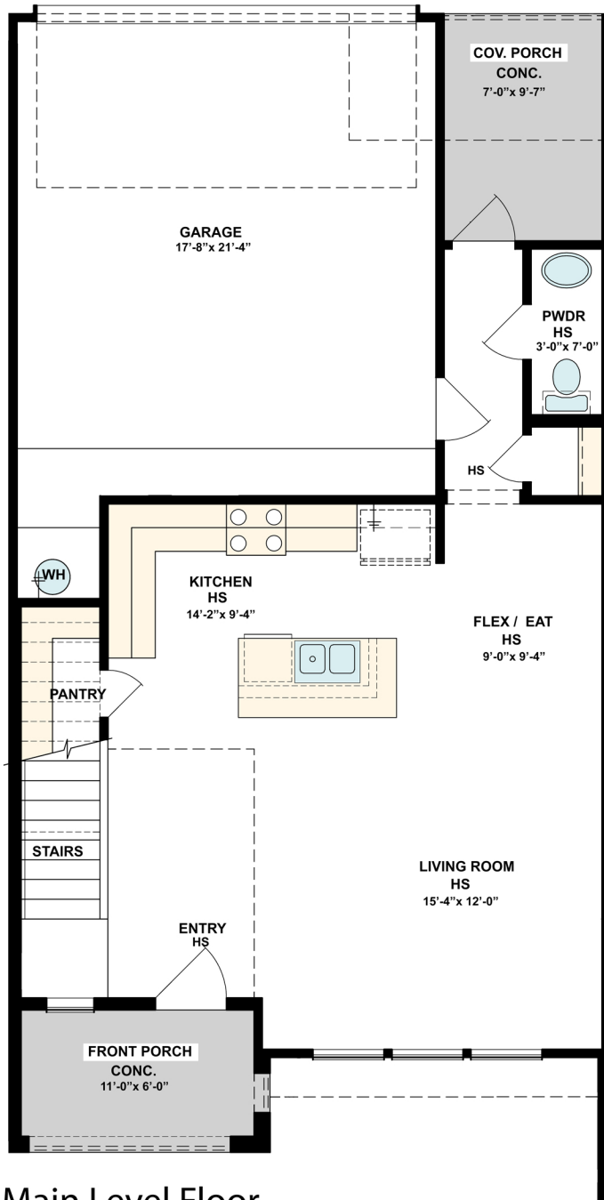
Main Level Floor
