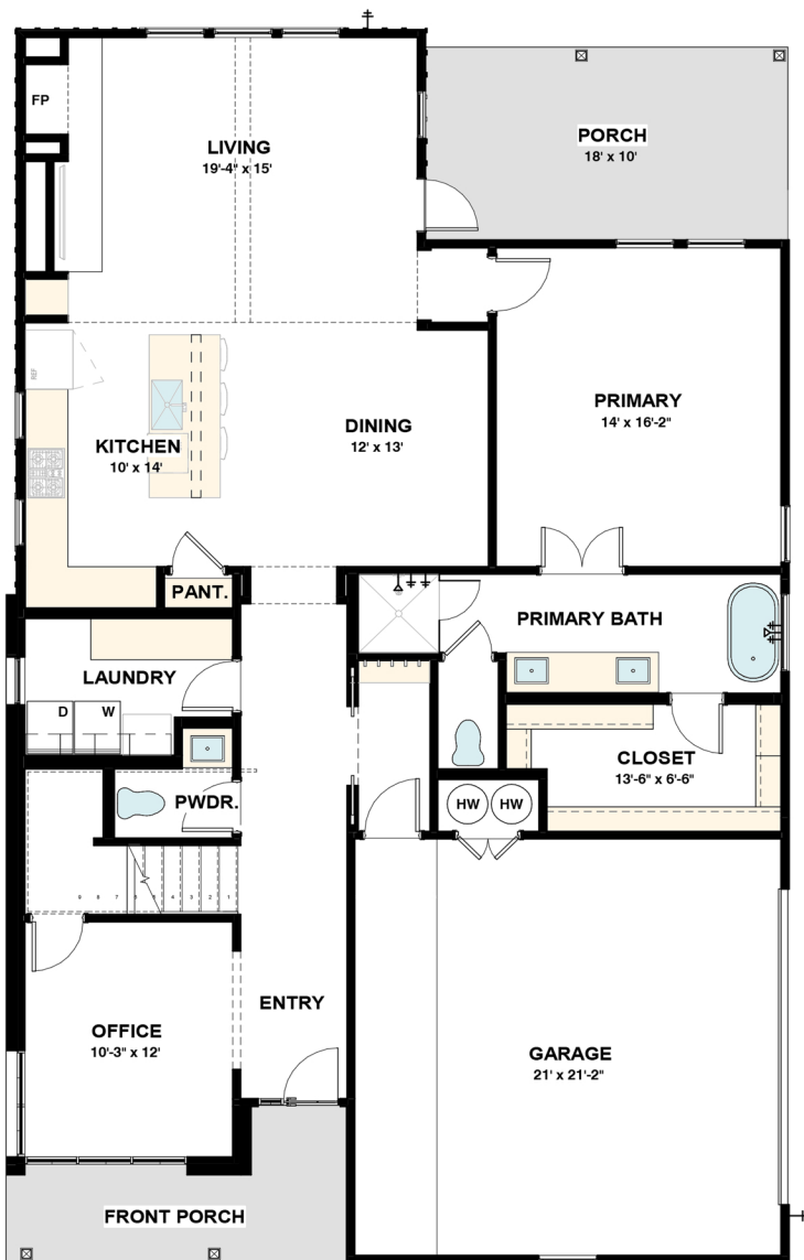
Main Level Floor
